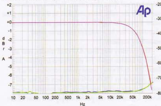
Krell Evolution 402e Frequency Response 1W 8ohm red (R,L) and distortion yellow (R) and green (L)
